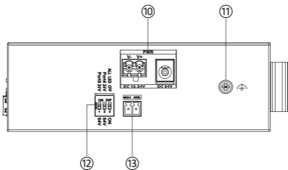
Figure 1-2 Side Panel
