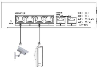
Figure 4-4 PD Connection
