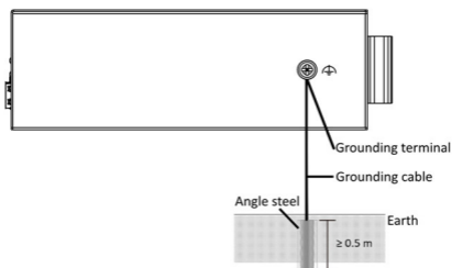
Figure 3-2 Grounding with Angle Steel
