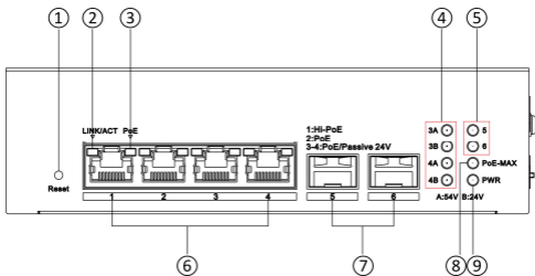
Figure 1-1 Front Panel
