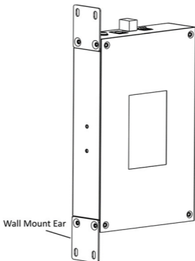
Figure 2-1 Wall-Mounted Installation
