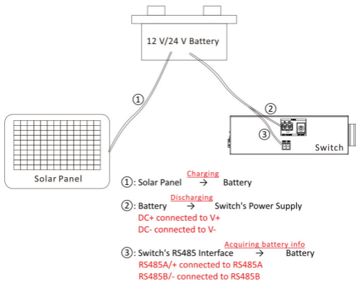
Figure 4-2 Power Connection
